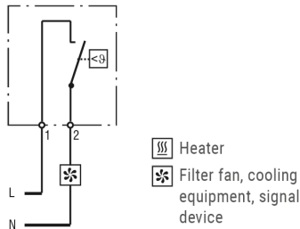
Thermostat KTS 111 (NO)
