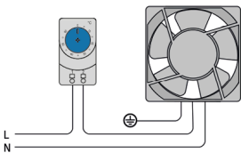
Connection examples
