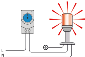
Thermostat KTS 111 (NO)
