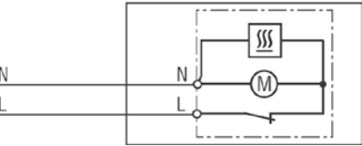
Connection diagram
