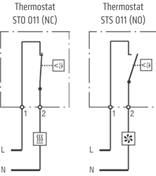
Connection diagrams
