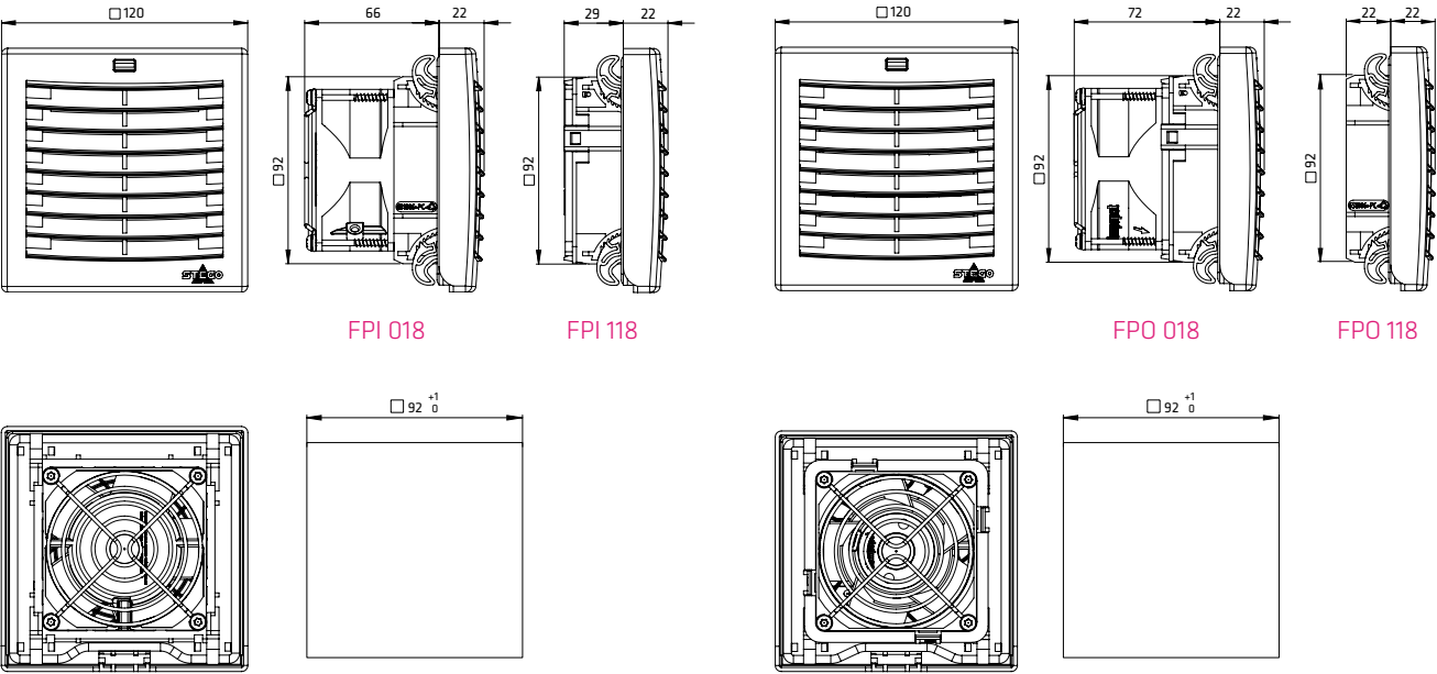
ENCLOSURE CUT-OUT
