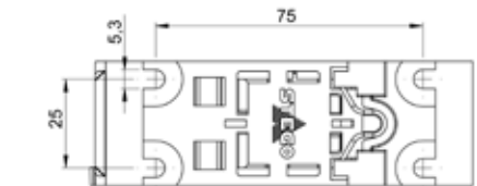
Universal mounting bracket for DIN rail and screw mounting
