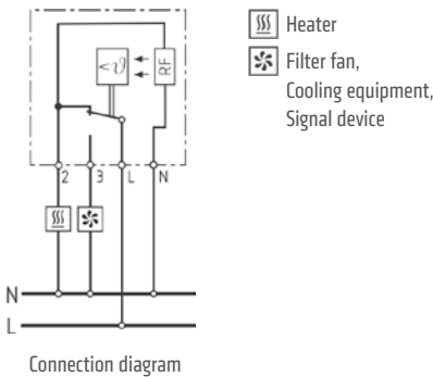
Connection diagram
