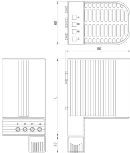
Heater CSF 060
