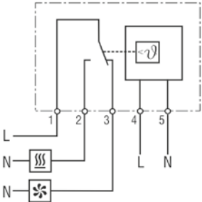
Connection diagram
