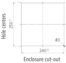
Enclosure cut-out
