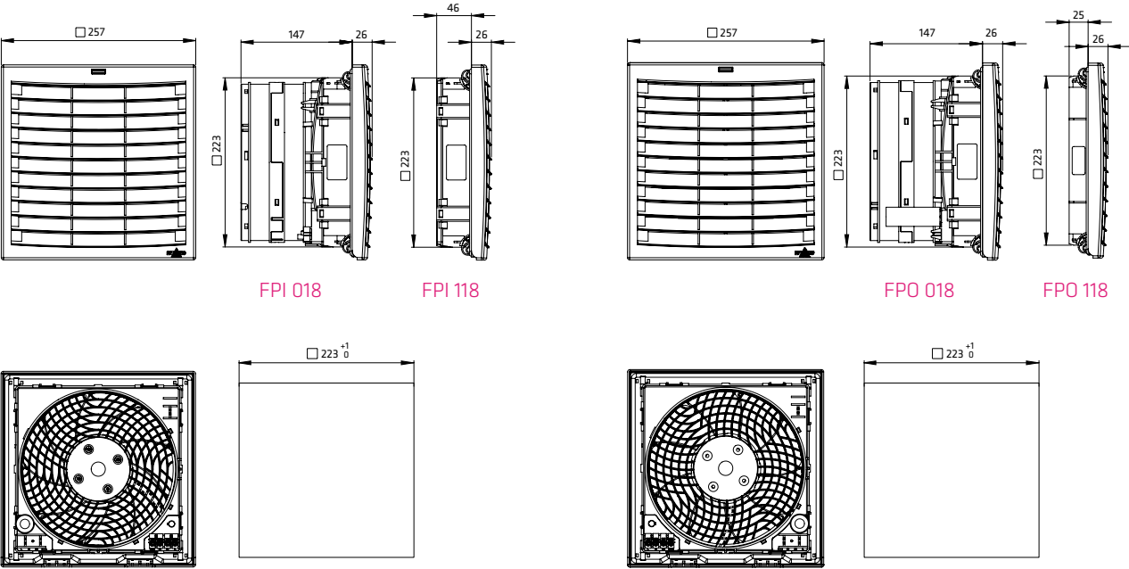
ENCLOSURE CUT-OUT
