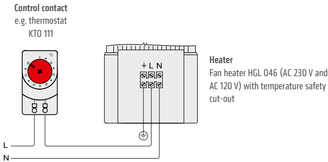
Example of connection
