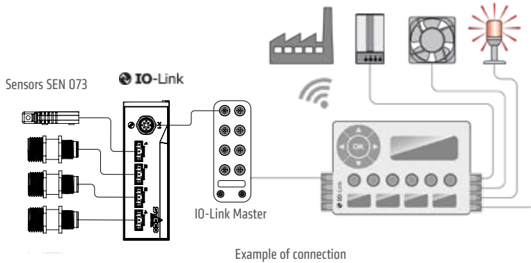
Example of connection
