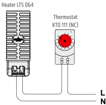
Example of connection
